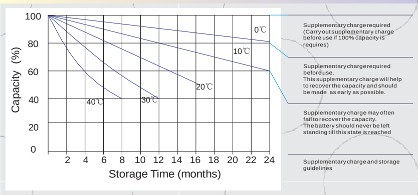
Storage characteristic
